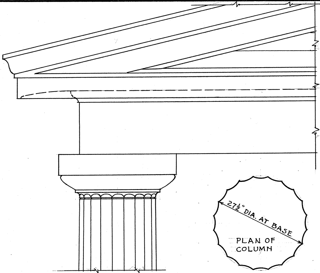
DETAILS OF MAIN CORNICE AND COLUMN SCALE \frac{3}{4} " = 1 FOOT
